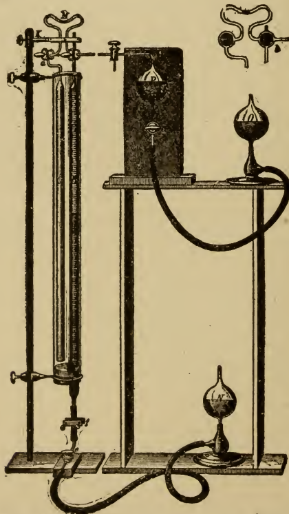
Fig. 126. APPARATUS FOR GAS ANALYSIS.
